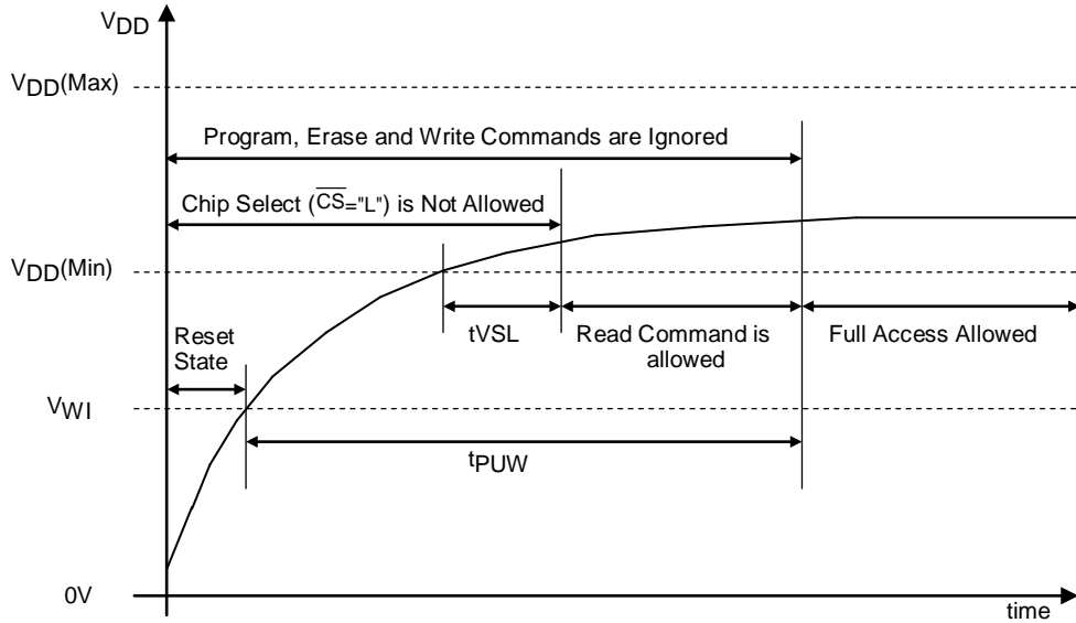
Figure 25. Power-on Timing
